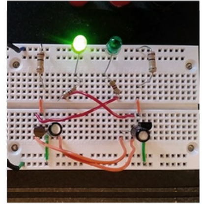
LED BLINKER WITH VARIABLE TIME DELAY
